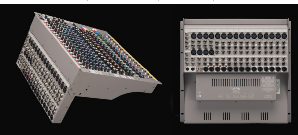
ProRack rear panel shown in full open and closed positions.
