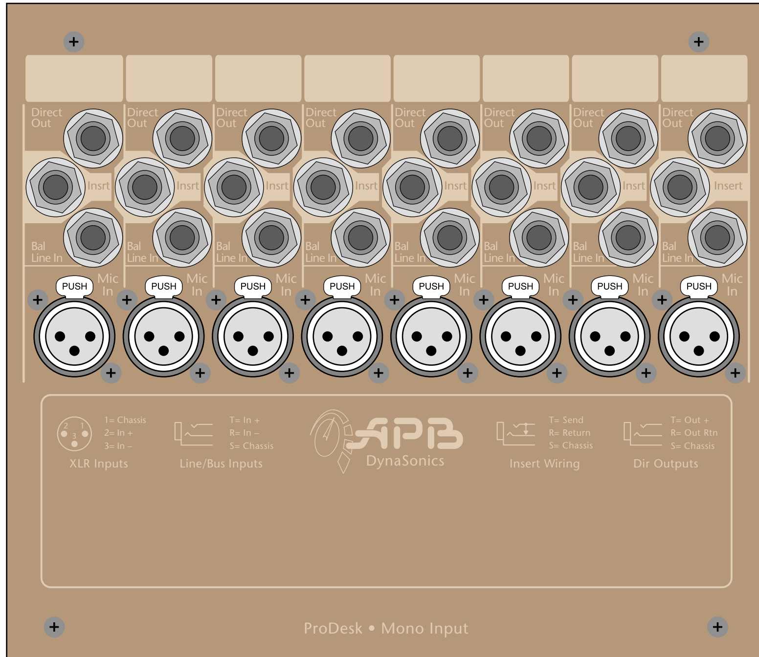
ProDesk Input Connector Panel
