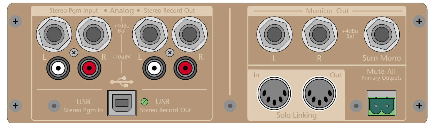
ProDesk Master Interface Panel
